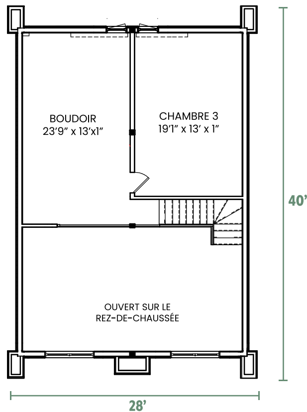
MEZZANINE
